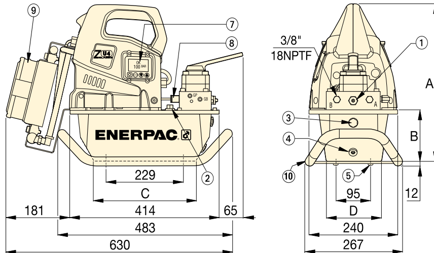
ZU4-Series with 4 and 6,6 litres reservoirs
