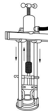
Bearing Puller shown with Crosshead Puller Attachment. ▶
