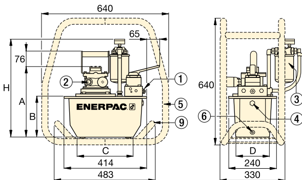
ZA4-Series Pumps with 4,0 - 6,6 litres reservoir
