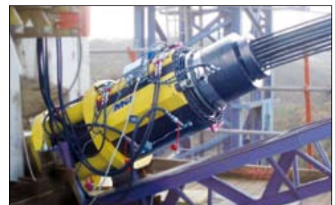
▼ Two concrete arches of this viaduct in Silleda, Spain are rotated and lowered by Enerpac Heavy Lifting Strand Jacking Systems.
